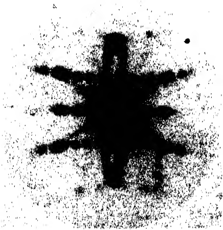
FIG. 6. X-RAY FIBER-BUNDLE PHOTOGRAPHS OF ASBESTOS. (FROM ASTBURY, "FUNDAMENTALS OF FIBRE STRUCTURE.")
